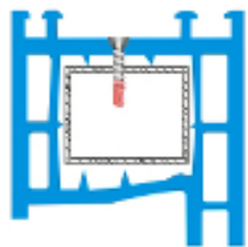
3 Hinges Fastening: Flat Head
