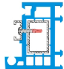
4 Handle Locking: Flat Head
